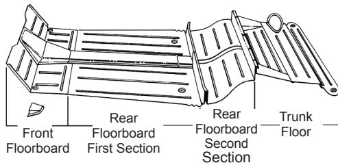
SEDAN FLOOR PAN ILLUSTRATION (4) Individual Parts
